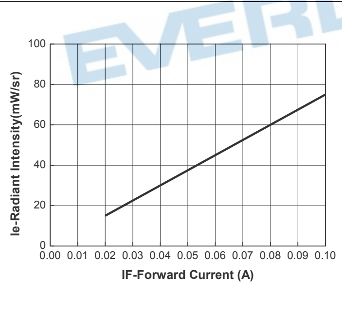
Radiant Intensity vs. Forward Current
