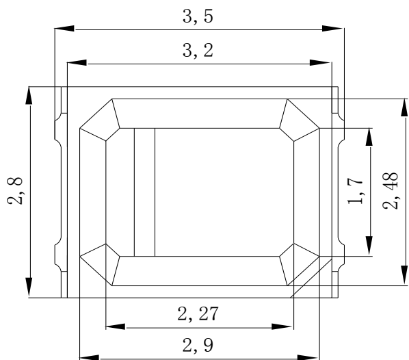
Fig.1-1 Top view
