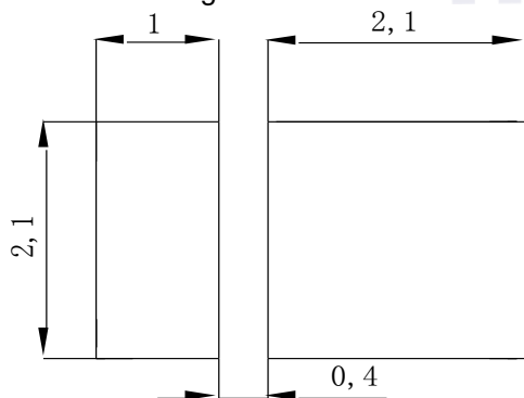
Fig.1-5 Soldering patterns
