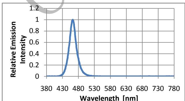
Fig.7- Spectrum Distribution
