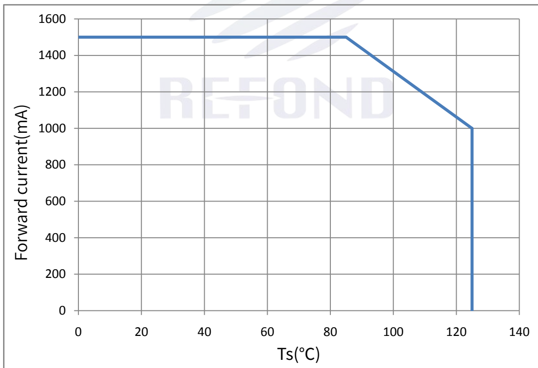
Fig 1-9 Ts Temperature Vs Forward Current 管脚温度与正向电流特性曲线 Tj ≤ 150°C
