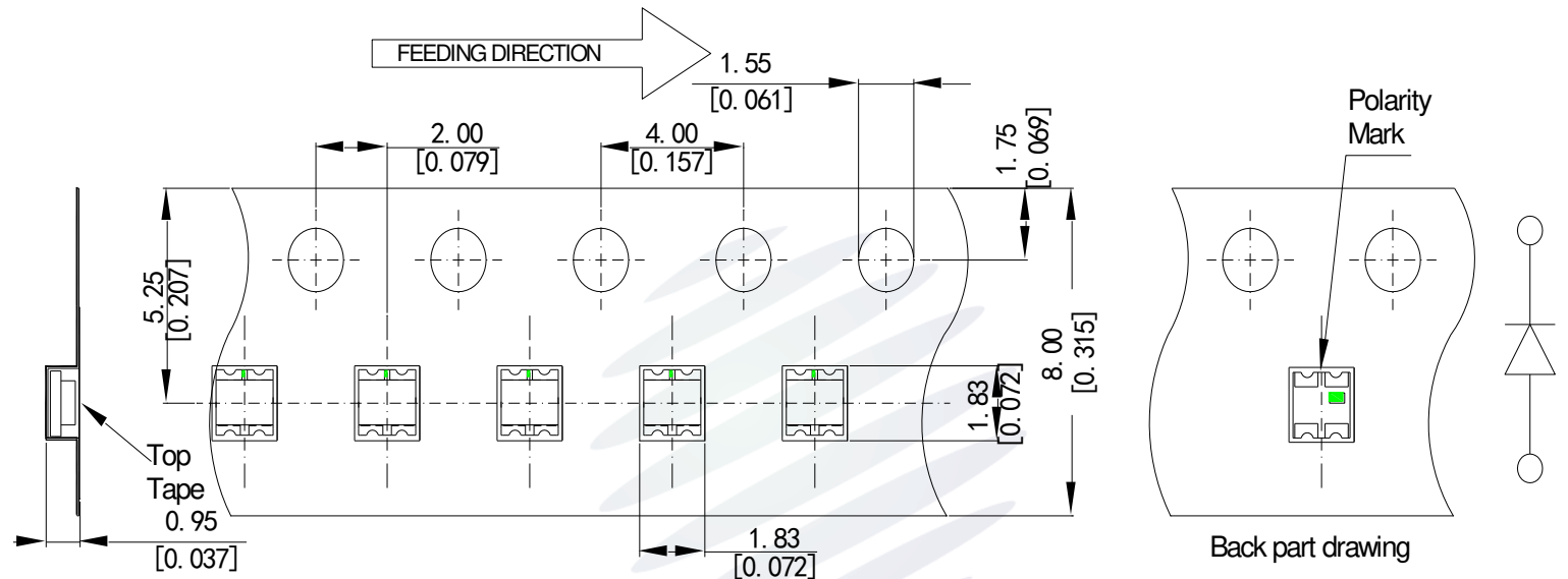
Fig.2-1 Carrier Tape Dimension 载带尺寸
