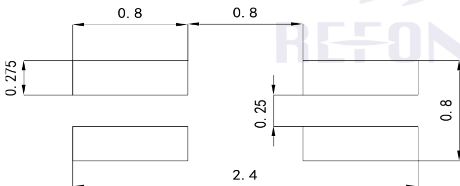
Fig.1-5 Soldering patterns 推荐焊盘
