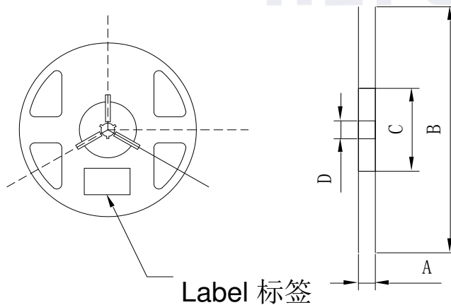
Fig.2-2 Reel 卷盘
