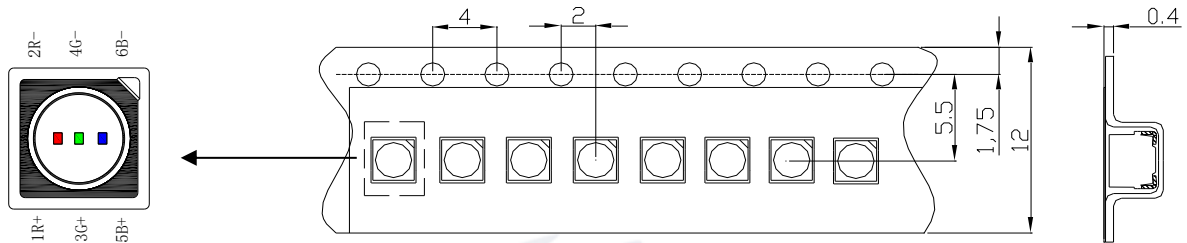
Fig.2-1 Carrier Tape Dimension 载带尺寸
