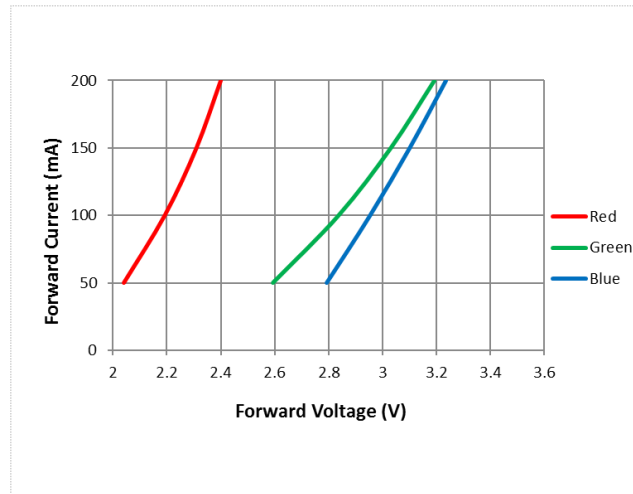
Fig 4. Forward Current vs. Forward Voltage, T_a = 25^{\circ}\text{C}
