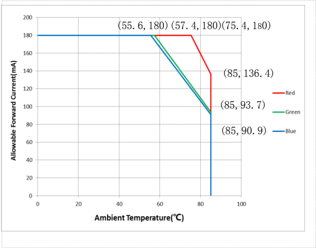
Fig 7. Ambient Temperature vs.Maximum Forward
