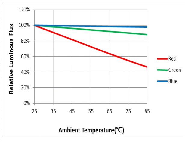
Fig 5. Ambient Temperature vs. Relative Luminous flux (IF=150mA)
