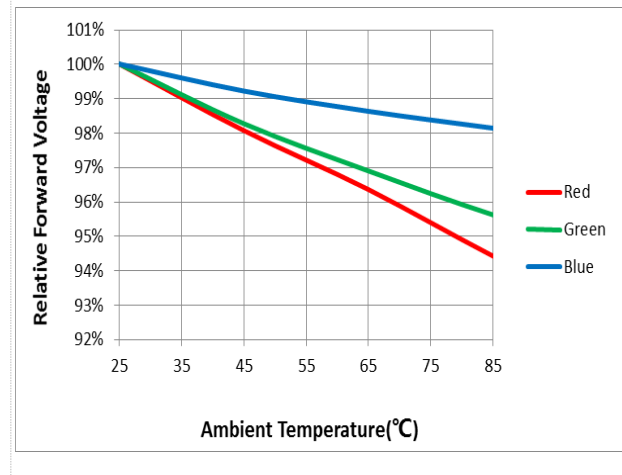
Fig 6. Ambient Temperature vs. Relative Forward Voltage (IF=150mA)
