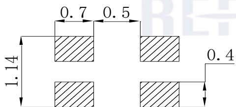
Fig.1-5 Soldering patterns 推荐焊盘
