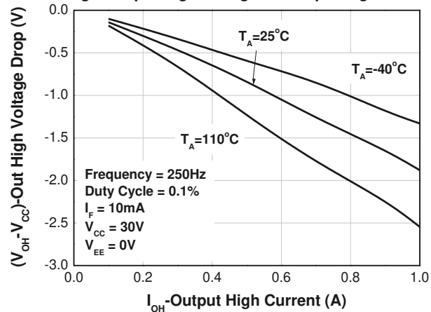
Fig.2 Output High Voltage vs. Output High Current
