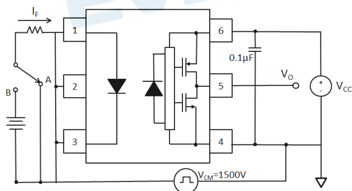
Fig. 22 CMR Test circuit
