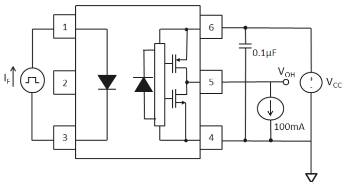
Fig. 17 V_{OH} Test circuit
