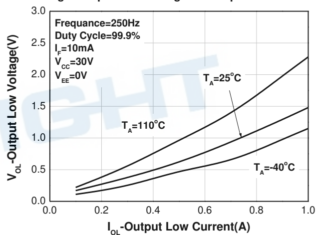
Fig.4 Output Low Voltage vs. Output Low Current
