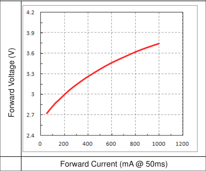
Forward Voltage vs. Forward Current (T solder pad =25°C)
