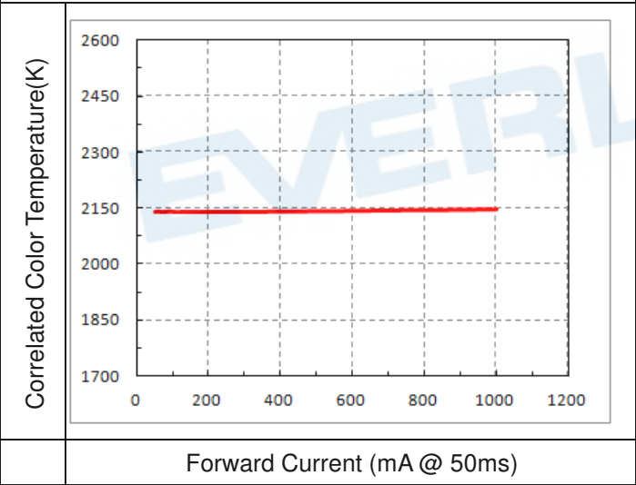
CCT vs. Forward Current (T soldering pad =25°C)
