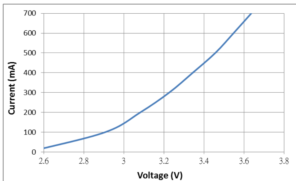
Fig 4. Forward Current vs. Forward Voltage
