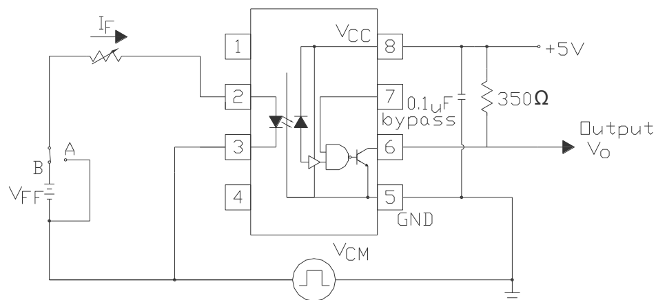
Fig. 14 Test circuit Common mode Transient Immunity
