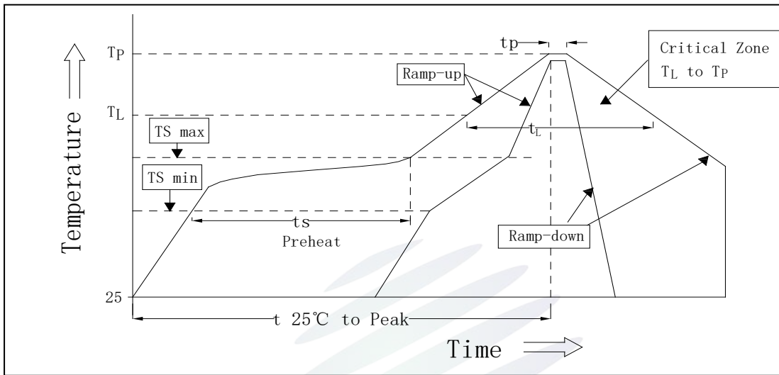
Fig.3-1SMT Reflow Soldering Instructions SMT 回流焊说明
