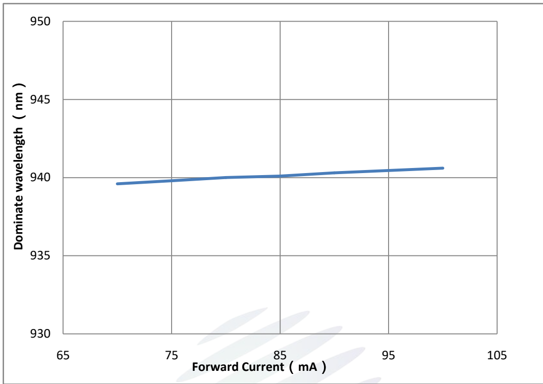
Fig. 1-13 Forward current vs.Dominate wavelength (Ts=25°C)正向电流与主导波长特性曲线(Ts=25°C)
