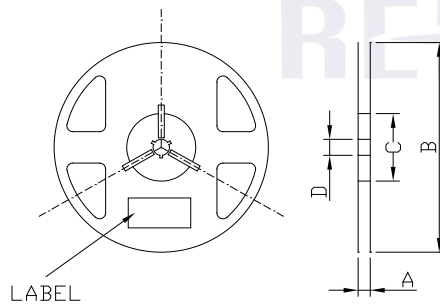
Fig.2-2 Reel Dimension 卷盘尺寸
