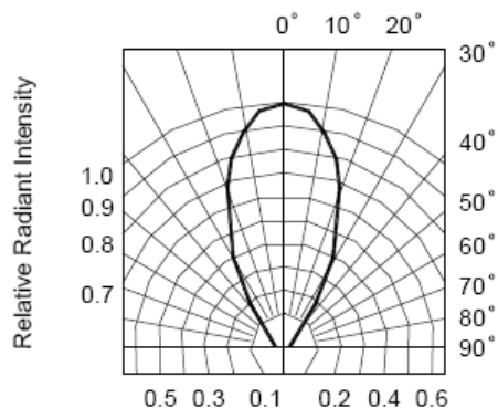
FIG. 5 RADIATION DIAGRAM
