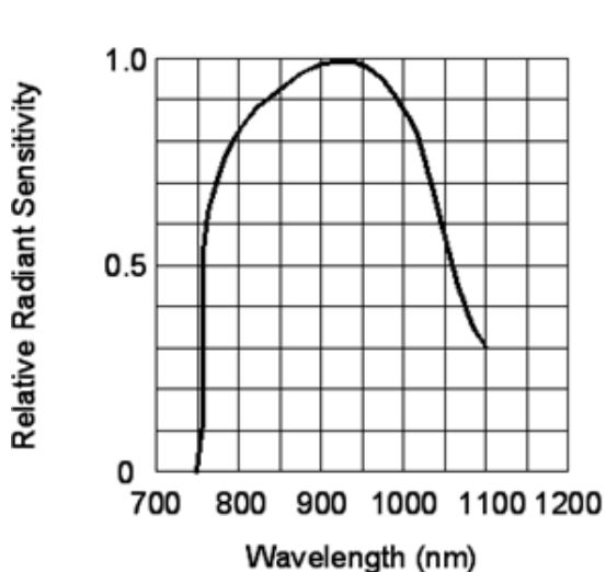
FIG.5 SPECTRAL SENSITIVITY
