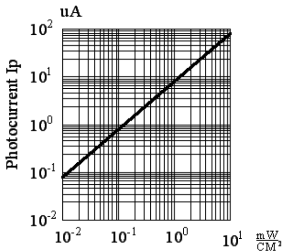
Fig6 PHOTOCURRENT VS IRRADIANCE \lambda = 940nm
