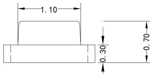
Fig.1-2 Side view 侧面视图
