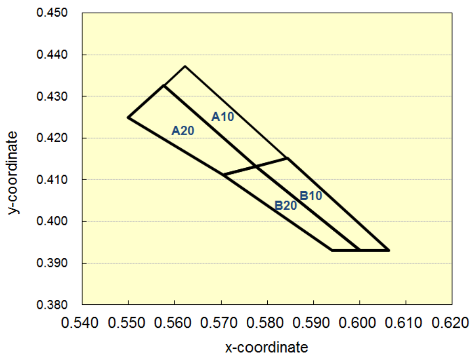
1931 CIE chromaticity
