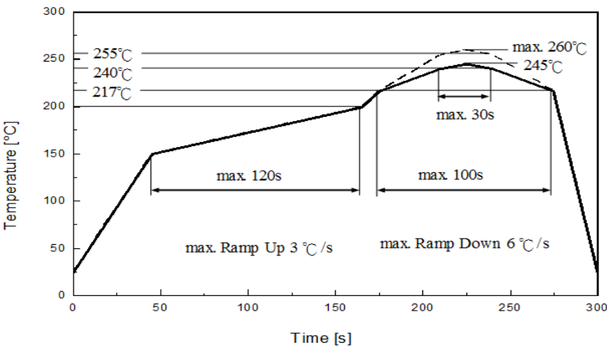
Soldering Condition (Reference: IPC/JEDEC J-STD-020D)
