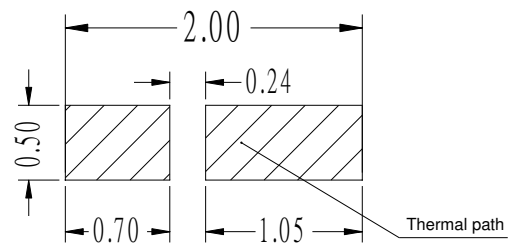
Soldering Pad
