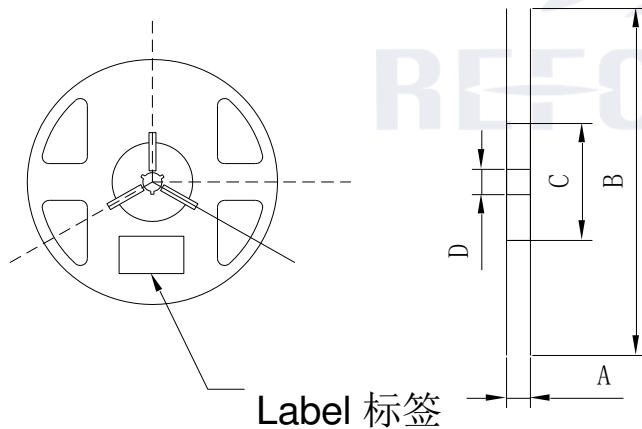
Fig.2-2 Reel 卷盘
