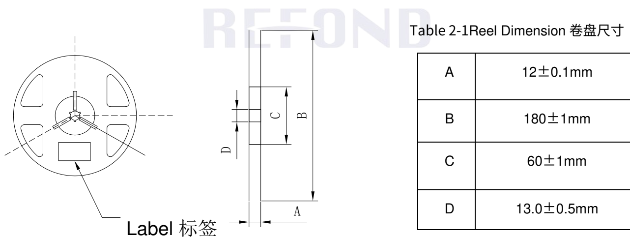
Fig.2-2 Reel Dimension 卷盘尺寸
