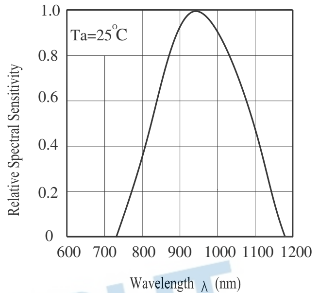
Spectral Sensitivity
