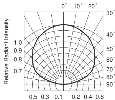
FIG.6 SENSITIVITY DIAGRAM
