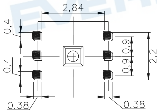
Bot. view
