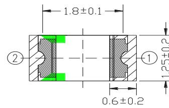
Recommend Soldering Pad
