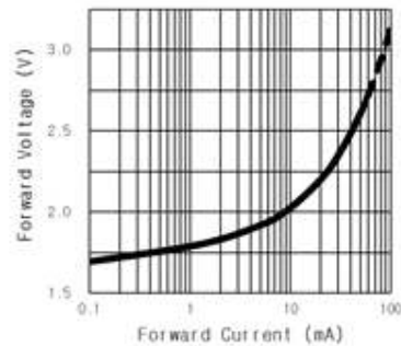
Fig. 3 FORWARD VOLTAGE V.S. FORWARD CURRENT
