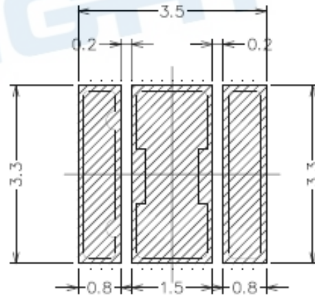
Soldering patterns
