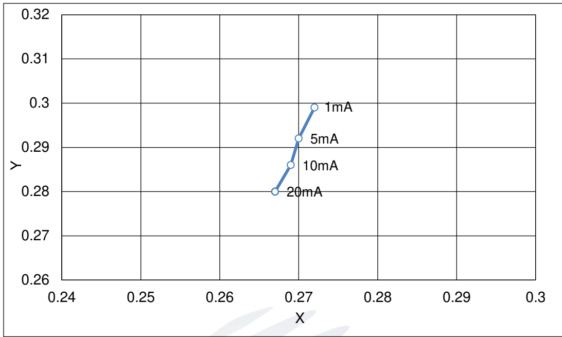
Fig.1-11 Forward Current Vs Dominant Wavelength (Ta=25°C) 正向电流与主波长关系曲线
