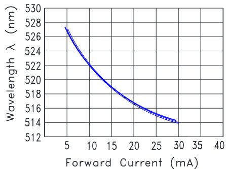
Fig.5 Wavelength \lambda (nm) VS. Forward Current (mA)
