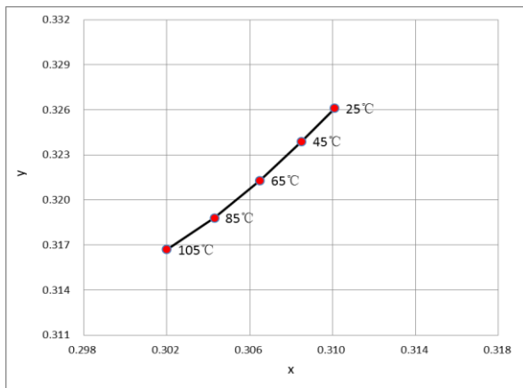
Fig 7. Chromaticity Coordinates vs. Ambient Temperature (IF=30mA)
