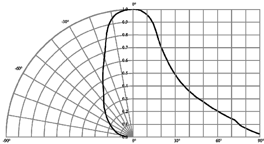
Fig 3. Radiation Characteristics
