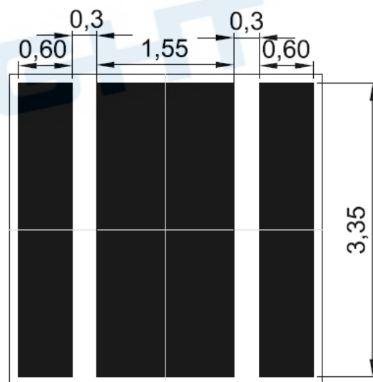
Soldering patterns
