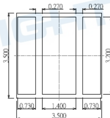
Soldering patterns
