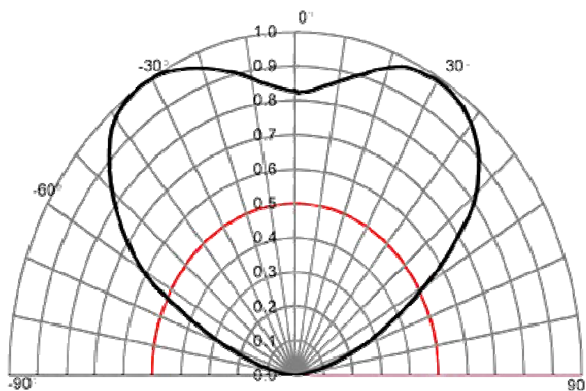
Fig 2. Radiation Characteristics
