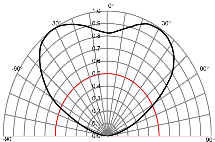
Fig 5. Radiation Characteristics
