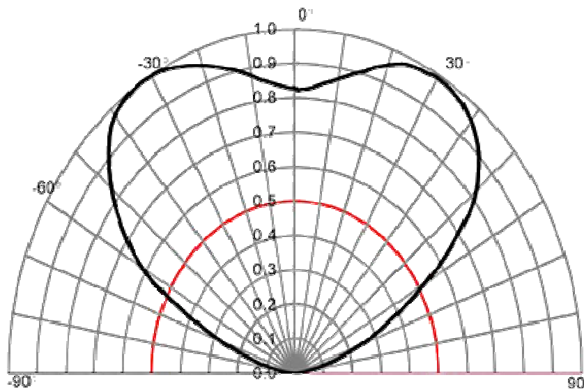
Fig 2. Radiation Characteristics
