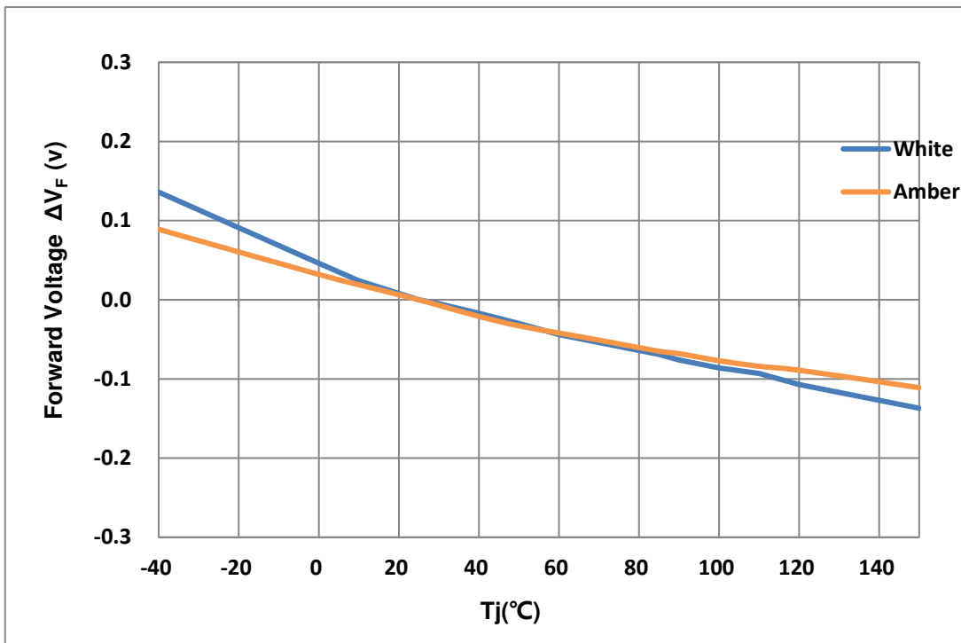
Fig. 1-12 Voltage Shift Vs Junction Temperature 电压偏移与结温特性曲线
