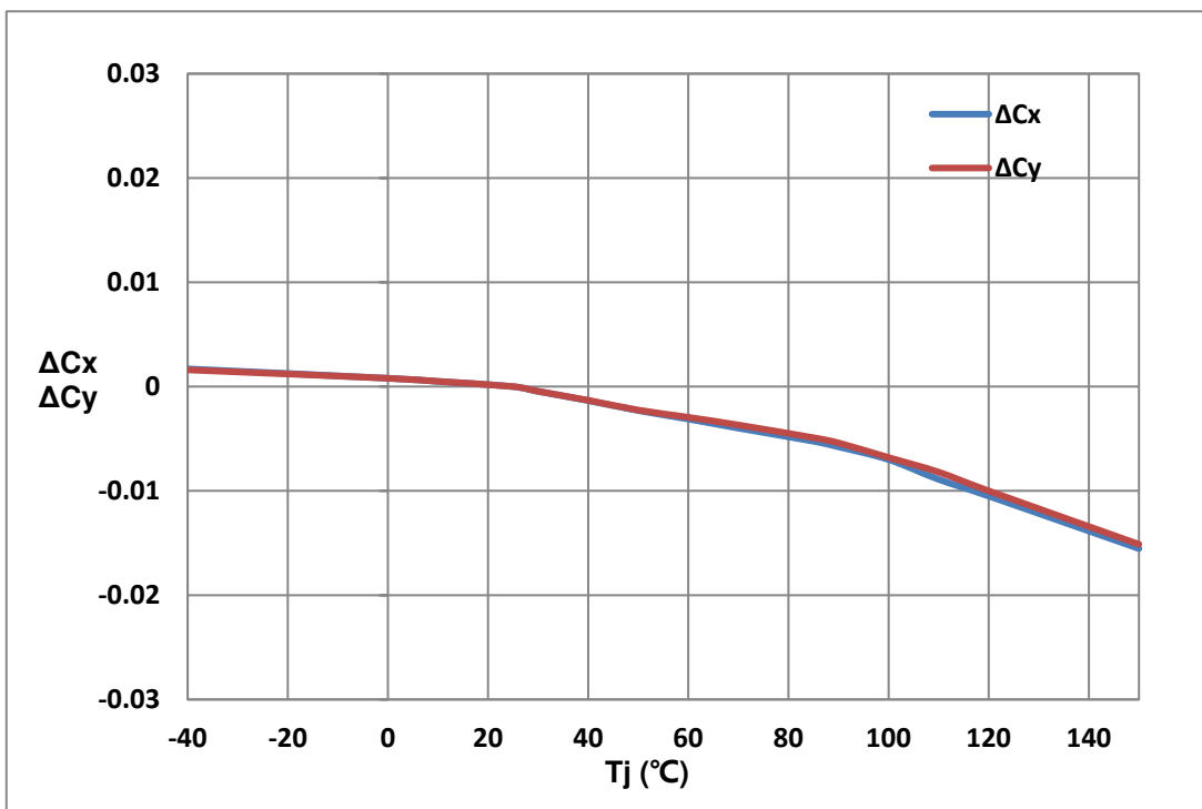
Fig. 1-14 Chromaticity Coordinate Shift Vs Junction Temperature (White) 色坐标偏移与结温特性曲线 (白光)
