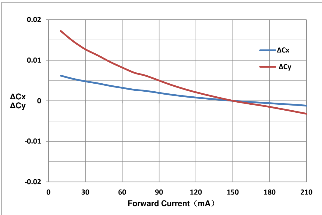
Fig. 1-16 Chromaticity Coordinate Shift Vs Forward Current (White) 色坐标偏移与正向电流特性曲线 (白光)
