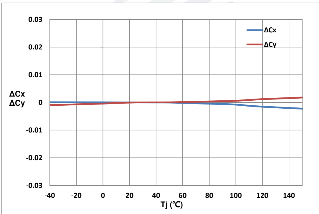
Fig. 1-15 Chromaticity Coordinate Shift Vs Junction Temperature (Amber) 色坐标偏移与结温特性曲线 (琥珀光)
