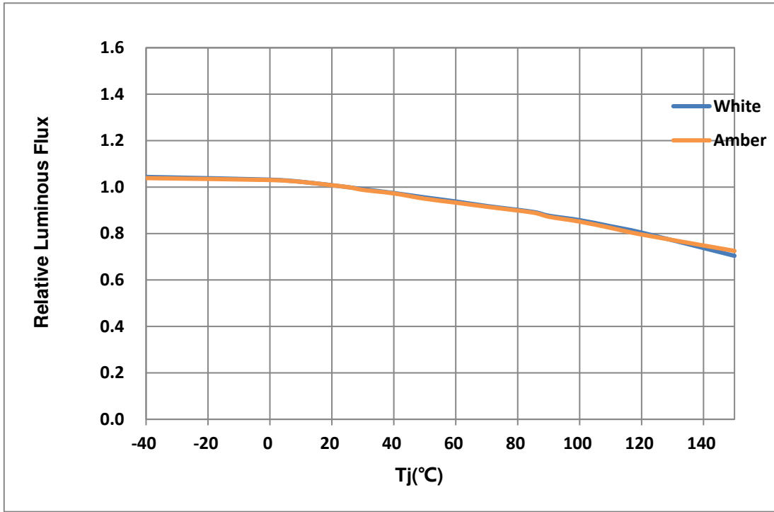
Fig. 1-10 Junction Temperature Vs Relative Luminous Flux 结温与相对光通量特性曲线
