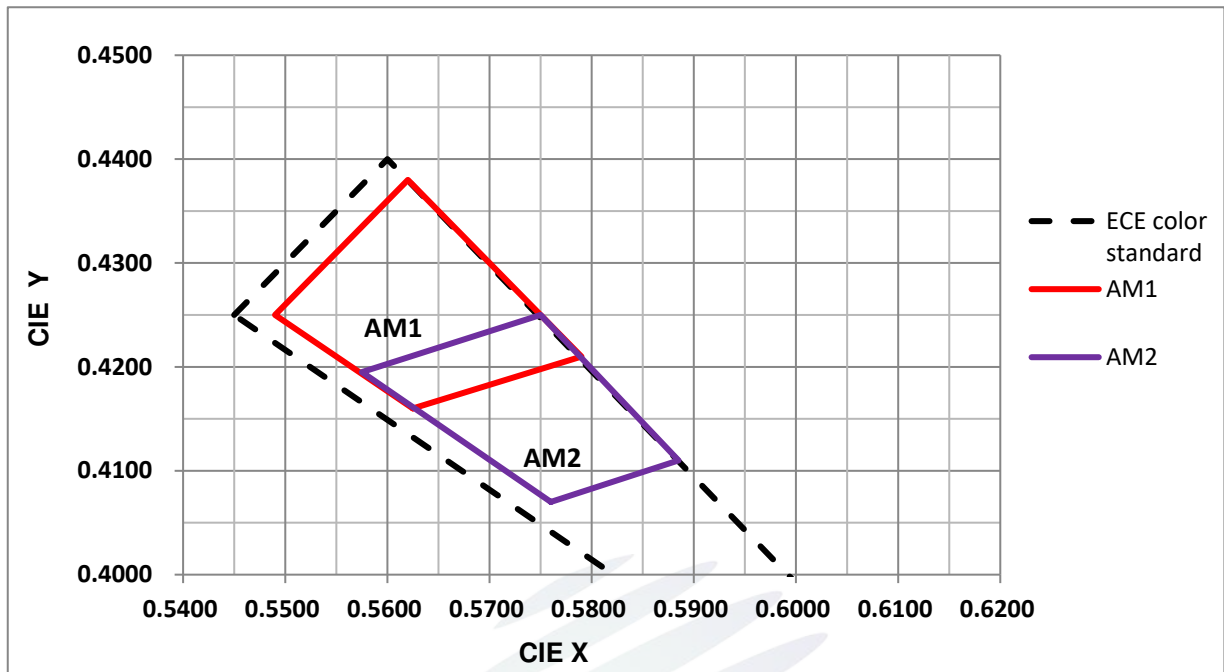
Fig. 1-7 The C.I.E Chromaticity Diagram CIE(Amber) CIE色度图 (琥珀光)
