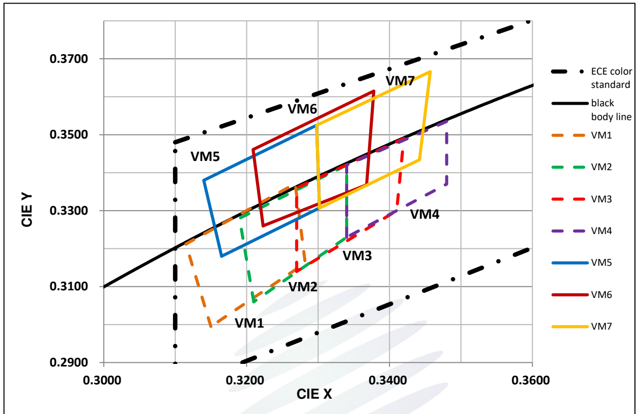
Fig. 1-6 The C.I.E Chromaticity Diagram CIE(White) CIE色度图 (白光)
