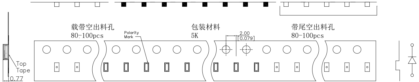
Fig.2-1 Carrier Tape Dimension 载带尺寸
