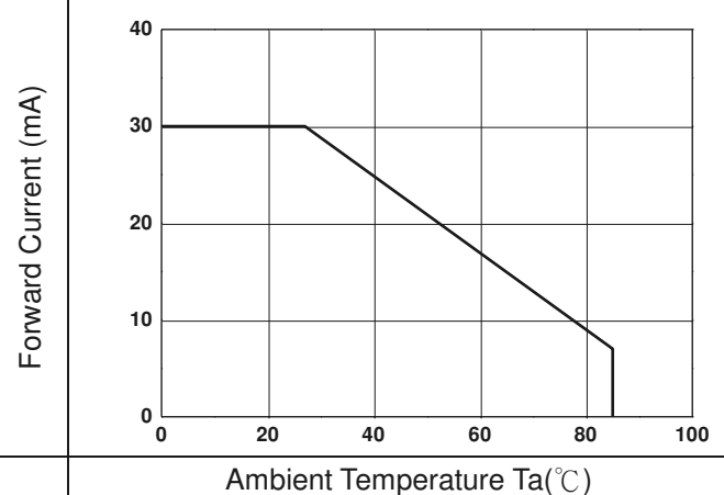
Forward Current vs. Ambient Temp.
