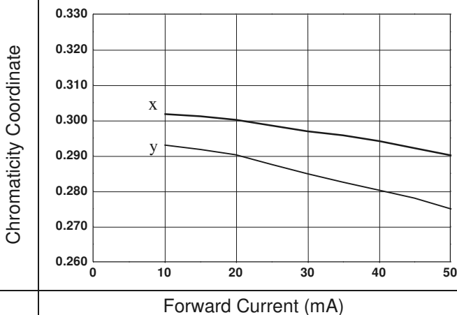
Chromaticity Coordinate vs. Forward Current (Ta=25°C)
