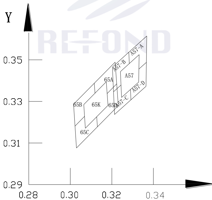
Fig 1-6 The C.I.E Chromaticity Diagram CIE色度图
