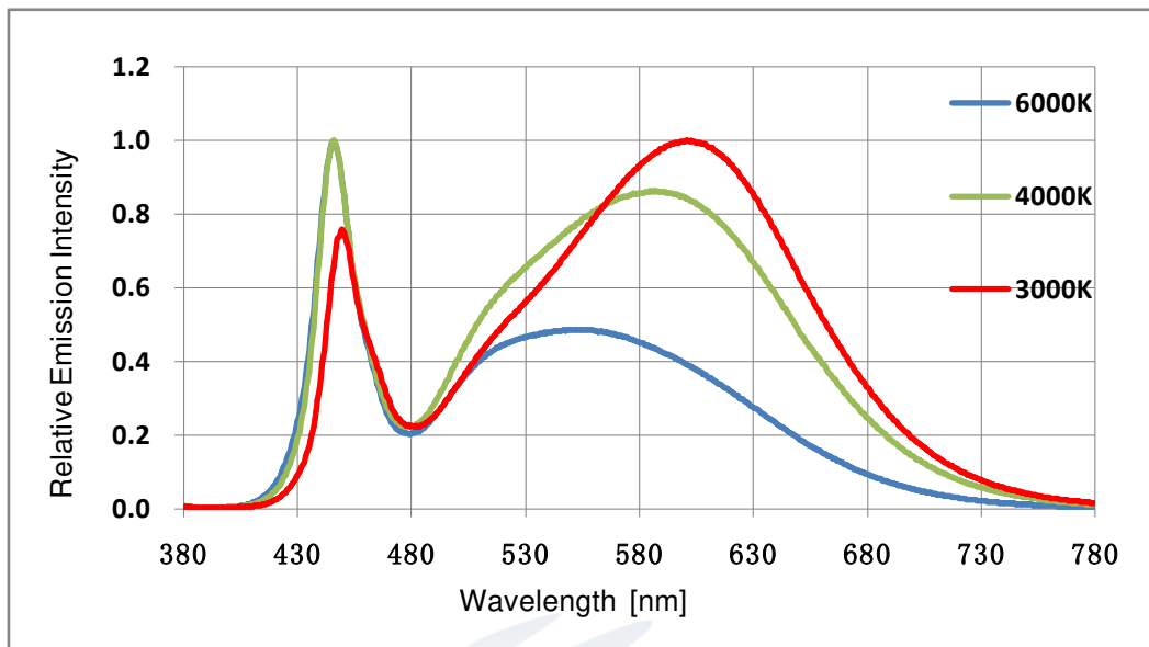
Fig 1-13 Spectrum Distribution光谱分布特性曲线
