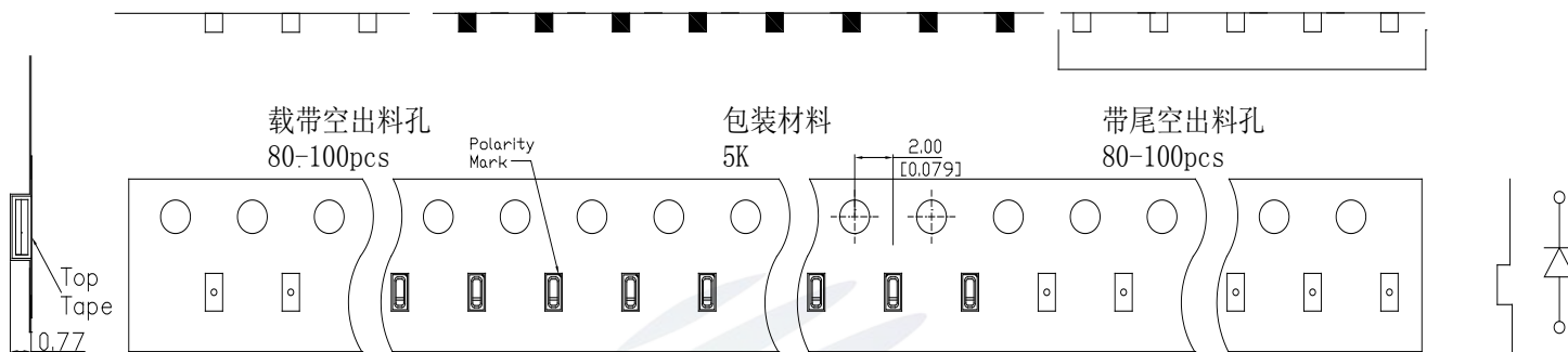
Fig.2-1 Carrier Tape Dimension 载带尺寸
