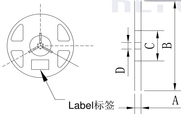
Fig.2-2 Reel Dimension 卷盘尺寸
