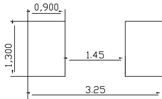
Soldering Patterns
