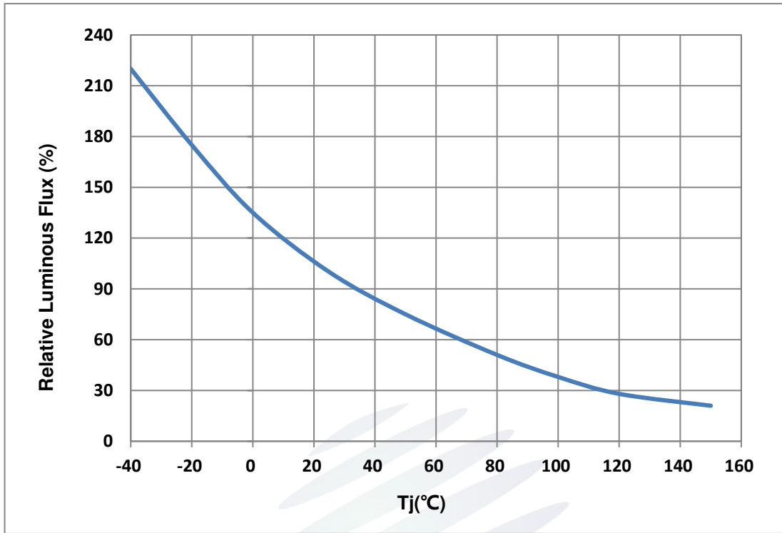
Fig. 1-8 Junction Temperature Vs Relative Luminous Flux 结温与相对光通量特性曲线
