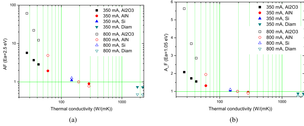
Fig. 6: Acceleration factor induced by replacing the AlN (193 W/(m·K)) carrier with the other carriers for current levels of 350 and 800 mA. (a) E_A = 2.5 eV activation energy (logarithmic Y scale). (b) E_A = 1.05 eV (linear Y scale).
