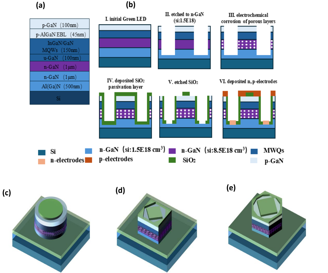
Figure 1. The detailed fabrication process flow of the porous Micro-LEDs. (a) Schematic diagram of the wafer structure. (b) schematic process flow for the formation of porous Micro-LEDs. Schematic structure of the porous Micro-LEDs. (c) circular Micro-LED structure. (d) square Micro-LED structure. (e) hexagonal Micro-LED structure.
